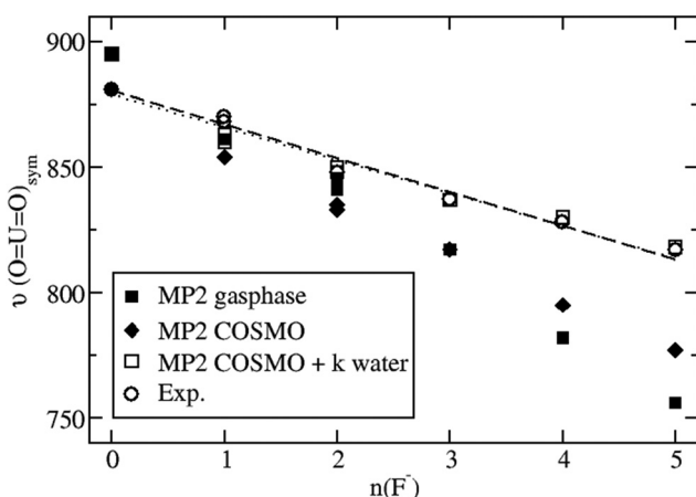
Fig. 3 Symmetric \text{UO}_2^{2+} stretching frequencies \nu(\text{O}=\text{U}=\text{O})_{\text{sym}} of [\text{UO}_2(\text{H}_2\text{O})_m\text{F}_n]^{2-n} complexes depending on the number n ( \text{F}^- ) of fluoride ligands. MP2 results for the gas phase and aqueous solution, modeled by COSMO as well as k explicitly treated water molecules and COSMO, in comparison to experimental values. The nearly linear dependence is illustrated by dashed and dotted lines for the MP2 COSMO + k water and experimental data sets, respectively.
