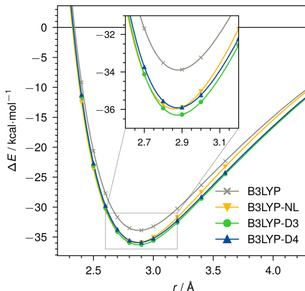
Fig. 4 Dissociation curve of Ac 3+ –Ar for B3LYP/def2-TZVP without dispersion correction, with NL, D3, or D4.
