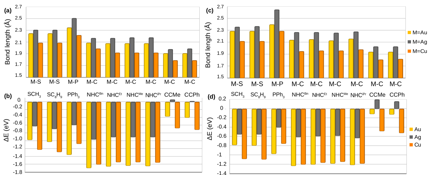
Fig. 2 Bond length M-L (Å) and binding energy (eV) calculated by PBE (shown in (a) and (b)) and BEEF-vdW (shown in (c) and (d)) for the M-L complexes. Table S2 contains the numeric values.
