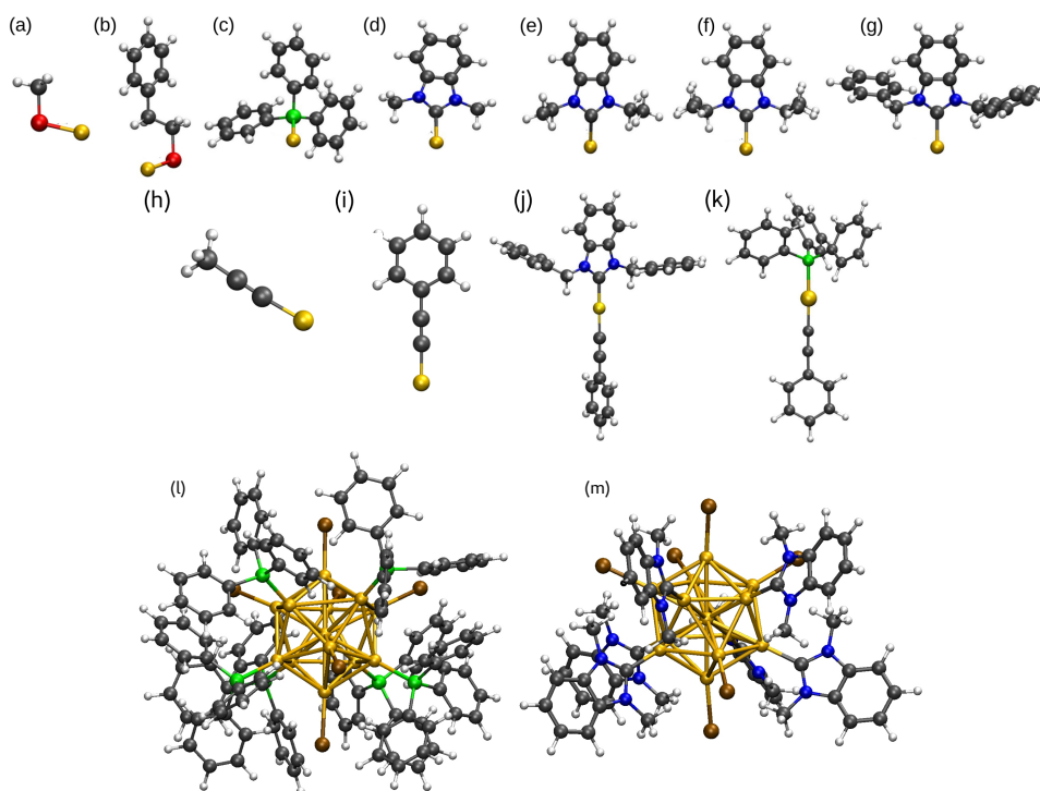
Fig. 1 Molecular structures of PBE optimized M-L complexes (a-i), L 1 -M-L 2 (j and k), and two PPh 3 and NHC Me protected metal clusters (l and m, respectively). (a) Au-SCH 3 , (b) Au-SC 8 H 9 , (c) Au-PPh 3 , (d) Au-NHC Me , (e) Au-NHC Et , (f) Au-NHC iPr , (g) Au-NHC Bn , (h) Au-CCMe, (i) Au-CCPh, (j) NHC Bn -Au-CCPh 3 , (k) PPh 3 -Au-CCPh, (l) [Au 13 (PPh 3 ) 6 Br 6 ] - , (m) [Au 13 (NHC Me ) 6 Br 6 ] - . Au, yellow; S, red; C, black; H, white; P, green; N, blue; Br, brown. The optimized structures of Au-L, L 1 -Au-L 2 , and [Au 13 L 6 Br 6 ] - are representative of all M-L and L 1 -M-L 2 complexes and ligand protected metal clusters; the atom radius is not precise.
