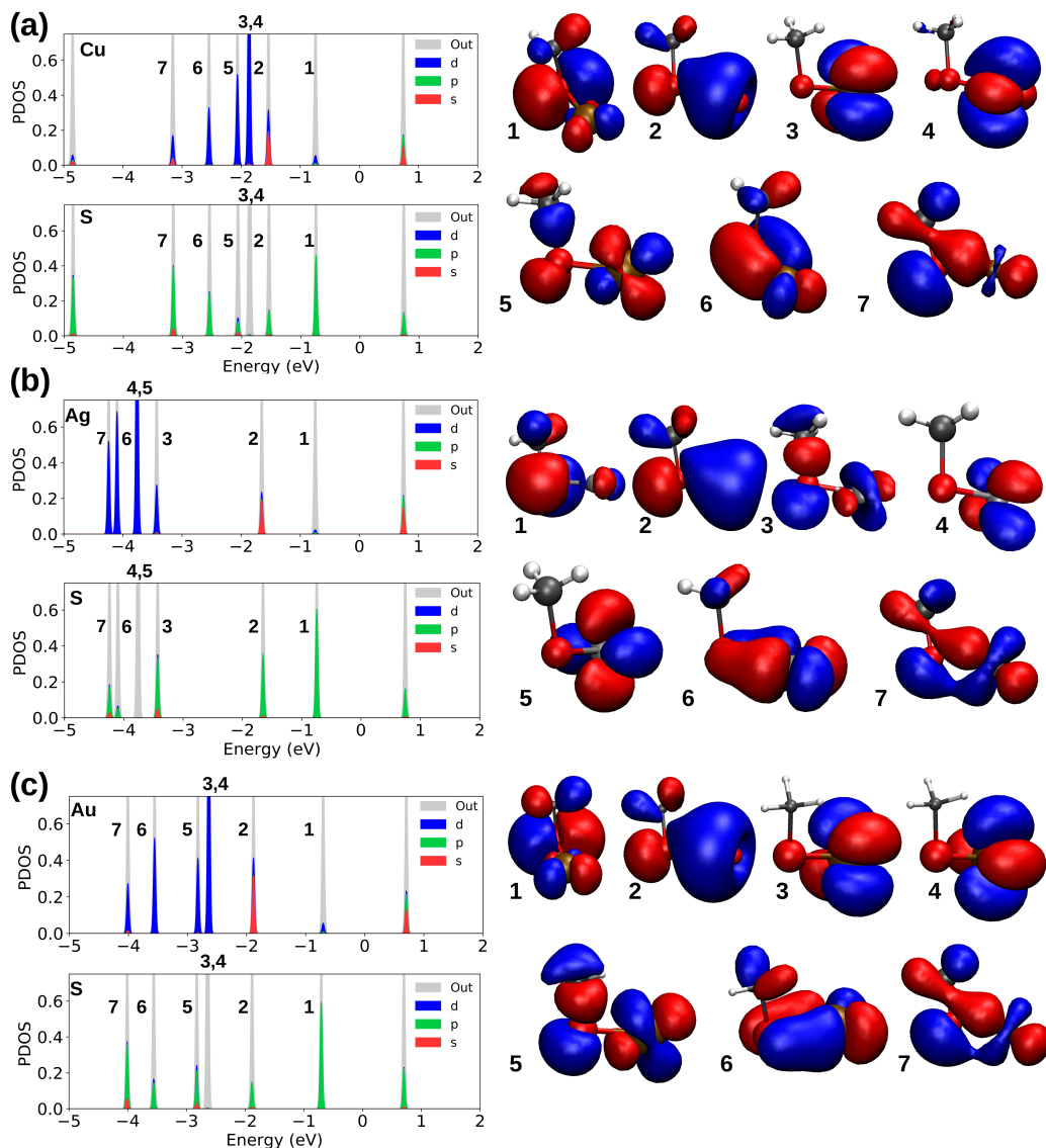
Fig. 3 Projected density of states along with the occupied molecular orbitals (the numbers 1 to 7 for refer to HOMO to HOMO-6) for (a) Cu-SCH 3 , (b) Ag-SCH 3 and (c) Au-SCH 3 . The HOMO-LUMO gaps (centered around zero) are 1.48, 1.49, and 1.41 eV for systems a through c, respectively.
