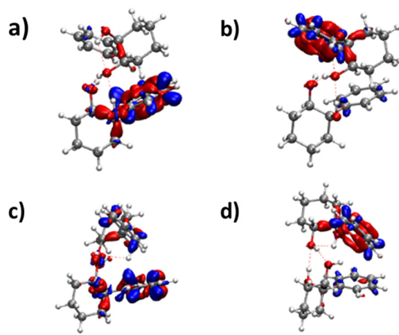
Fig. 9 Difference in electronic density for (a) the \text{S}_1 \leftarrow \text{S}_0 (b) \text{S}_2 \leftarrow \text{S}_0 transitions of the insertion homochiral dimer and (c) the \text{S}_1 \leftarrow \text{S}_0 (d) the \text{S}_2 \leftarrow \text{S}_0 transitions of the insertion heterochiral dimer.
