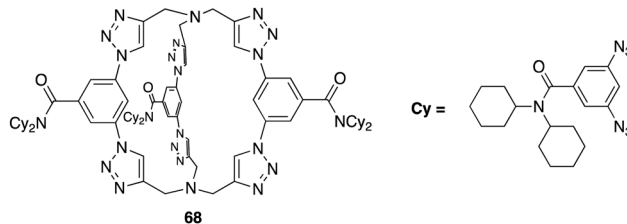
Fig. 34 General structure of cryptand-like triazolo cage ( 68 ) reported by Flood et al.
