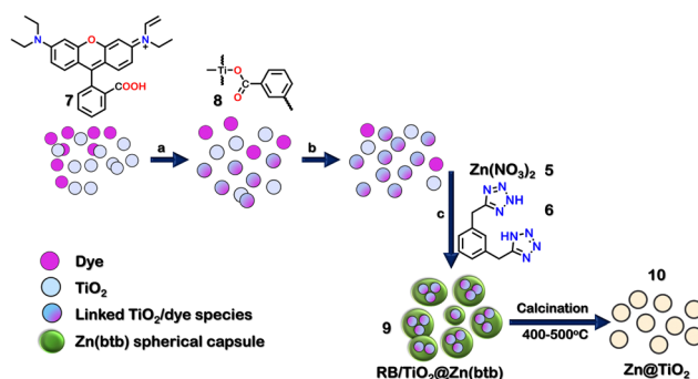
Fig. 4 Schematic representations for the formation of coordination polymer composite \text{RB/TiO}_2@\text{Zn(btb)} ( 9 ) [conditions: (a) 5 min sonication, (b) stirring at room temperature for 12 h, (c) methanolic solution of 5 was added with stirring at room temperature].
