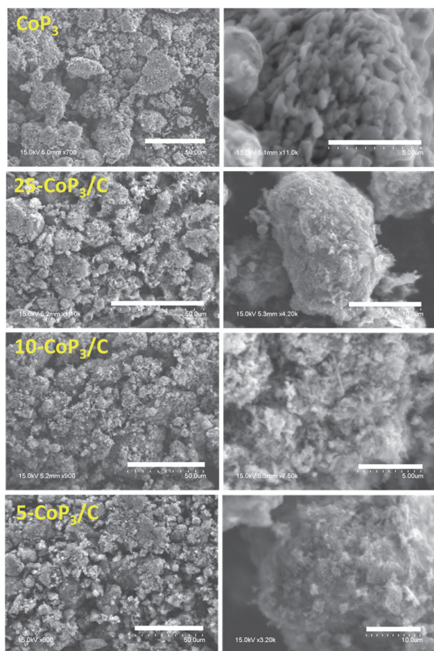
Fig. 4 Representative SEM images of CoP 3 and x\text{-CoP}_3/\text{C} ( x = 5, 10, 25 mol%) powders from reactions of x\text{-CoCl}_2/\text{C} and red phosphorus at 500 °C. Scale bars are 50 \mu\text{m} for all left images. Scale bar lengths for right images of CoP 3 and 10-CoP 3 /C are 5 \mu\text{m} and 25-CoP 3 /C and 5-CoP 3 /C are 10 \mu\text{m} .
