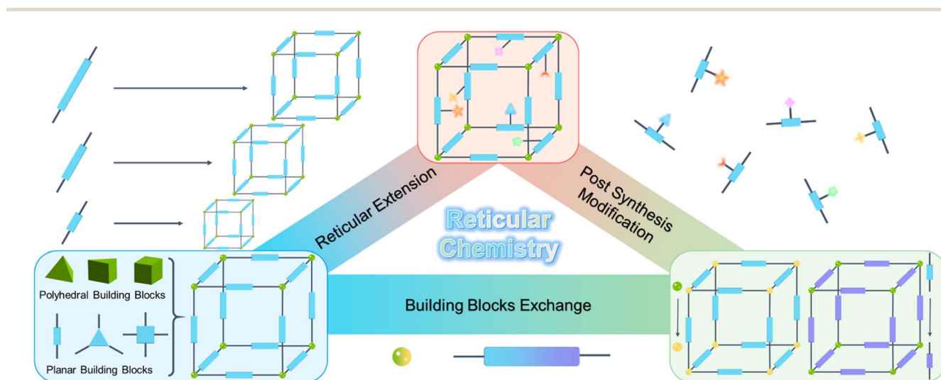
Fig. 3 Schematic illustration of reticular chemistry in 3D COFs.
