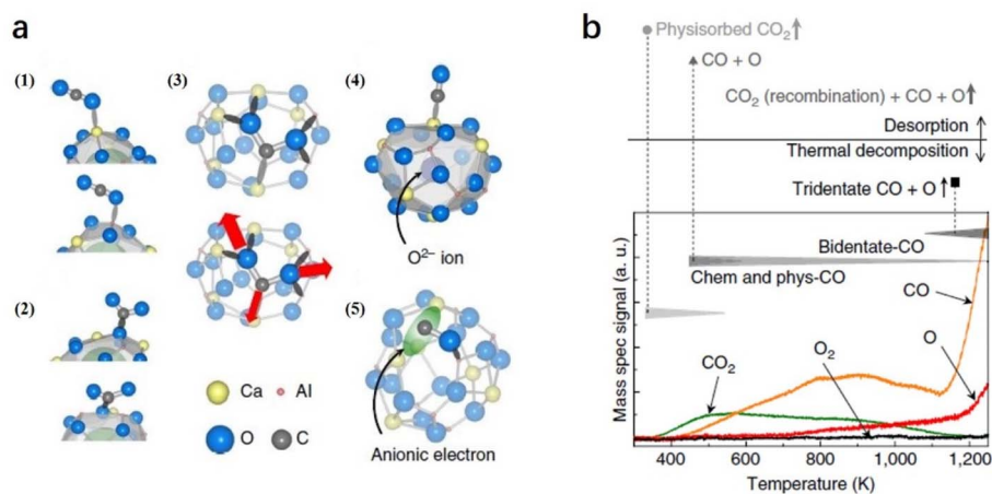
Fig. 15 (a) Geometrical configurations of a \text{CO}_2 molecule adsorbed on \text{C12A7:e}^- surface. (b) TPD curves of all desorption products from the \text{C12A7:e}^- surface after 2 L of exposure to \text{CO}_2 at RT with the proposed \text{CO}_2 desorption and decomposition sequence. The intensities of the curves were calibrated using sensitivity factors. Copyright 2013, Springer Nature.
