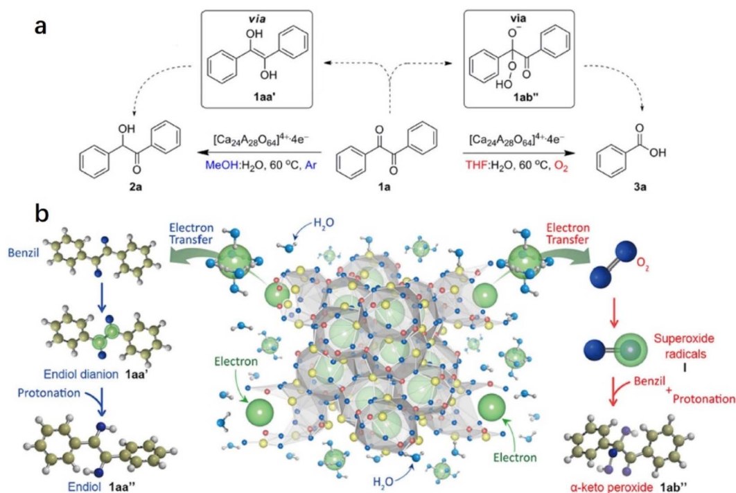
Fig. 14 Strategies for the chemoselective reduction and oxidation of 1,2-diketones using the \text{C12A7:e}^- electrode. (a) The chemoselective reduction and oxidation of benzil using the \text{C12A7:e}^- electrode. (b) Schematic illustration of the chemoselective reduction and oxidation of benzil by controlling the electron transfer pathway to benzil or \text{O}_2 via the release of electrons from the \text{C12A7:e}^- electrode via hydrolysis as well as the possible solvation of electrons by water molecules. Copyright 2015, Springer Nature.
