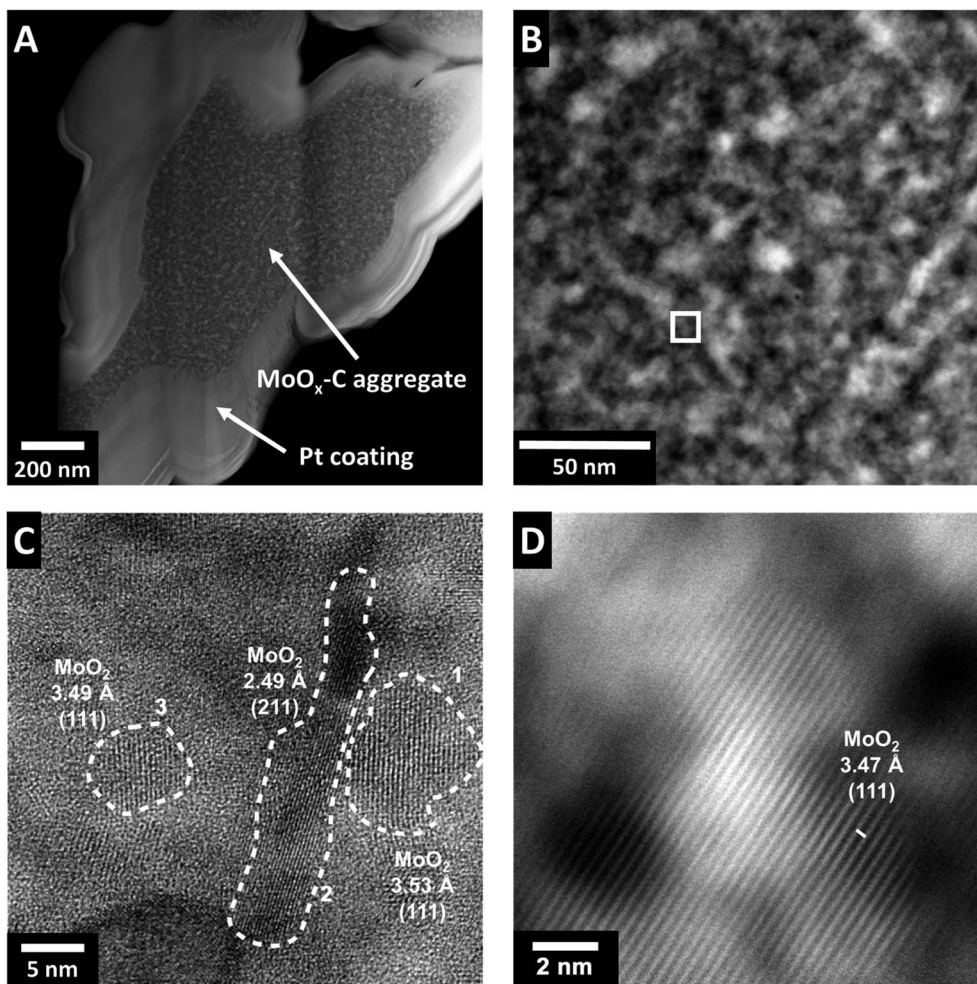
Fig. 4 Cross-sectional overview of the MoO x -C hybrid nanostructure. (A) HAADF-STEM micrograph of MoO x -C showing microstructure with non-homogeneous particle composition. (B) Magnified micrograph showing phase Z-contrast variations in MoO x -C, (C) bright field STEM micrograph taken at the area indicated in (B). The crystalline domains are highlighted and measurements of planar spacings are indicated on the image. Lattice spacings in regions 1, 2, and 3 are in good agreement with the (111), (211), and (111) planes of MoO 2 , respectively. (D) High resolution HAADF-STEM image of monoclinic MoO 2 nanodomain.
