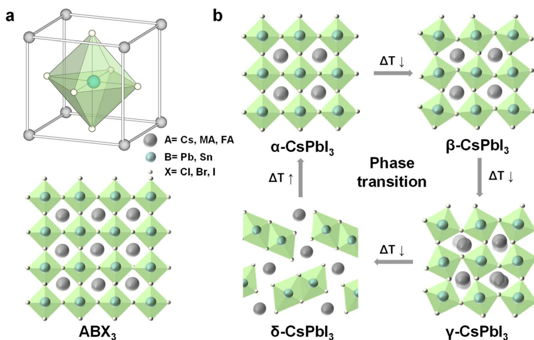
Fig. 2 (a) Illustration of the halide perovskite structure ABX_3 , A = \text{Cs}^+ , \text{CH}_3\text{NH}_2^+ ( \text{MA}^+ ), or \text{CH}_2(\text{NH}_2)_2^+ ( \text{FA}^+ ), B = \text{Pb}^{2+} , or \text{Sn}^{2+} ; X = \text{Cl}^- , \text{Br}^- , or \text{I}^- ; (b) crystal structure of the different \text{CsPbI}_3 phases and relative phase transitions. Reproduced from ref. 33 with permission from American Association for the Advancement of Science, copyright 2019.
