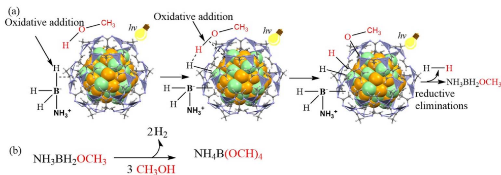
Scheme 1 Proposed mechanism for the AB methanolysis generating \text{H}_2 catalyzed by \text{Au}_{0.5}\text{Pd}_{0.5}\text{@ZIF-8} and accelerated by illumination with visible light.
