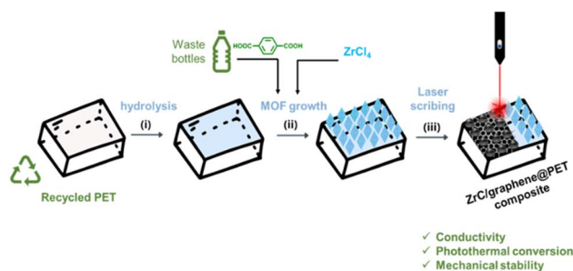
Fig. 1 Strategy for PET@LB-UiO-66 preparation from recycled PET: (i) PET hydrolysis, (ii) UiO-66 PET surface growth from waste PET bottle, and (iii) laser scribing process by 405 nm irradiation.
