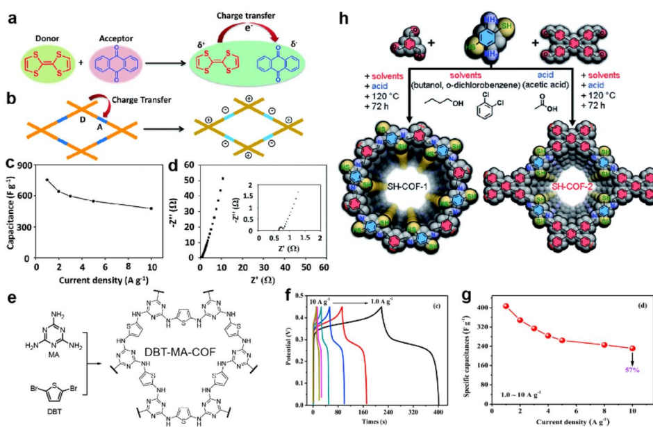
Fig. 12 Illustration of charge transfer (a) in tetrathiafulvalene and p -benzoquinone compounds and (b) in the donor–acceptor COF. (c) Capacitance vs. current density and (d) Nyquist plot (the inset is the magnified Nyquist plot) of the TTF-COF1 electrode in a three-electrode system. Reprinted from ref. 105. Copyright 2020, Royal Society of Chemistry. (e) Synthetic route and structure of DBT-MA-COF. (f) GCD curves and (g) Specific capacitances at various current densities of DBT-MA-COF. Reprinted from ref. 106. Copyright 2021, Elsevier. (h) Synthetic pathway of SH-COF-1 and SH-COF-2. Reprinted from ref. 107. Copyright 2022, Royal Society of Chemistry.
