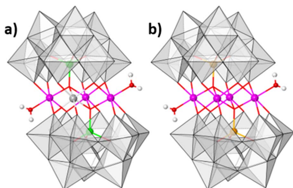
Fig. 7 Polyhedral representation of (a) [Co II (H 2 O) 2 Co II W VI (B- \alpha -Co IV W 9 O 34 ) 2 ] 12- ( Co 3 W-WS ) and (b) [Co II (H 2 O) 2 Co II (B- \alpha -PW 9 O 34 ) 2 ] 10- ( Co 4 -WS ). Colour code: pink: Co II in octahedral geometry; green: Co II in tetrahedral geometry; grey: W; orange: P; red: O; white: H; grey polyhedra: {WO 6 } units. Note that the internal belt positions of Co 3 W-WS have a 50 : 50 Co : W equal occupancy.
