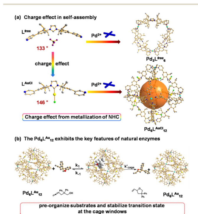
Fig. 1 (a) Charge effect of rigid NHC metallization-triggered supra-molecular configurations. (b) The Pd 6 L Au 12 cage presents the features of enzymatic catalysis at the cage window for gold-catalyzed cyclization of allenol. The structures of L free , L AuCl and Pd 6 L AuCl 12 are their single crystal X-ray structures. The structure of Pd 3 L free 6 is a modelled structure. Color coding: C: gray; N: dark blue; Au: yellow; Pd: light blue; Cl: bright green; B: dark green; F: violet; O: red; H: white.
