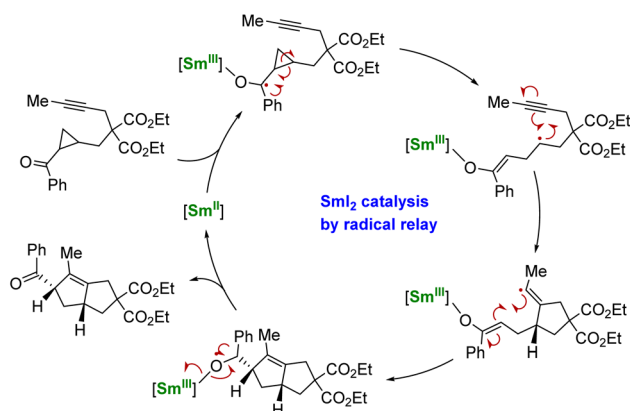
Scheme 5 Schematic catalytic cycle of the Sm II -induced electron transfer followed by cyclization and back electron transfer. 137
