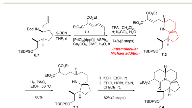
Scheme 7 Construction of the tricyclic core of halichlorine by Tomioka.
