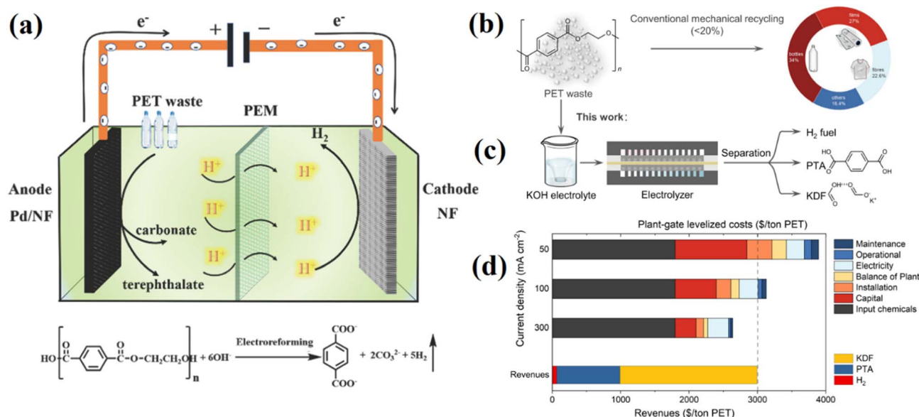
Fig. 14 (a) The electrocatalyst reforming process of PET into high value-added chemicals and \text{H}_2 fuel, 107 reproduced from ref. 107 with permission from [Royal Society of Chemistry], copyright [2021], (b) conventional route for PET recycling, (c) electrocatalytic PET upcycling to commodity chemicals and \text{H}_2 fuel, (d) technoeconomic analysis (TEA) of route I at different current density. 108 Reproduced from ref. 108 with permission from [Springer], copyright [2021].
