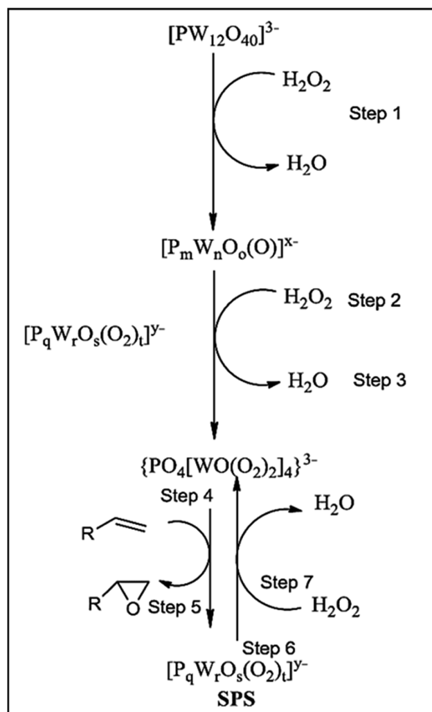
Scheme 23 Mechanism of active species formation. 12
