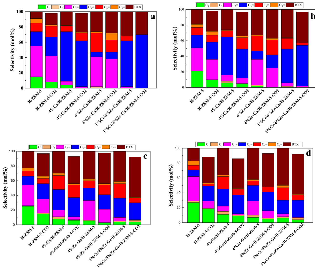
Fig. 7 Product distribution of bare and metal-doped H-ZSM-5 zeolites at (a) 400 °C, (b) 450 °C, (c) 500 °C, and (d) 550 °C. Reaction conditions: pressure, 1 bar; feed gas, \text{C}_3\text{H}_8/\text{N}_2 = 2.5/97.5 and \text{C}_3\text{H}_8/\text{CO}_2/\text{N}_2 = 2.5/5/92.5 ; flow rate, 75 \text{ mL min}^{-1} ; WHSV, 4 \text{ kg}_{\text{cat}} \text{ s mol}_{\text{C}_3\text{H}_8}^{-1} .
