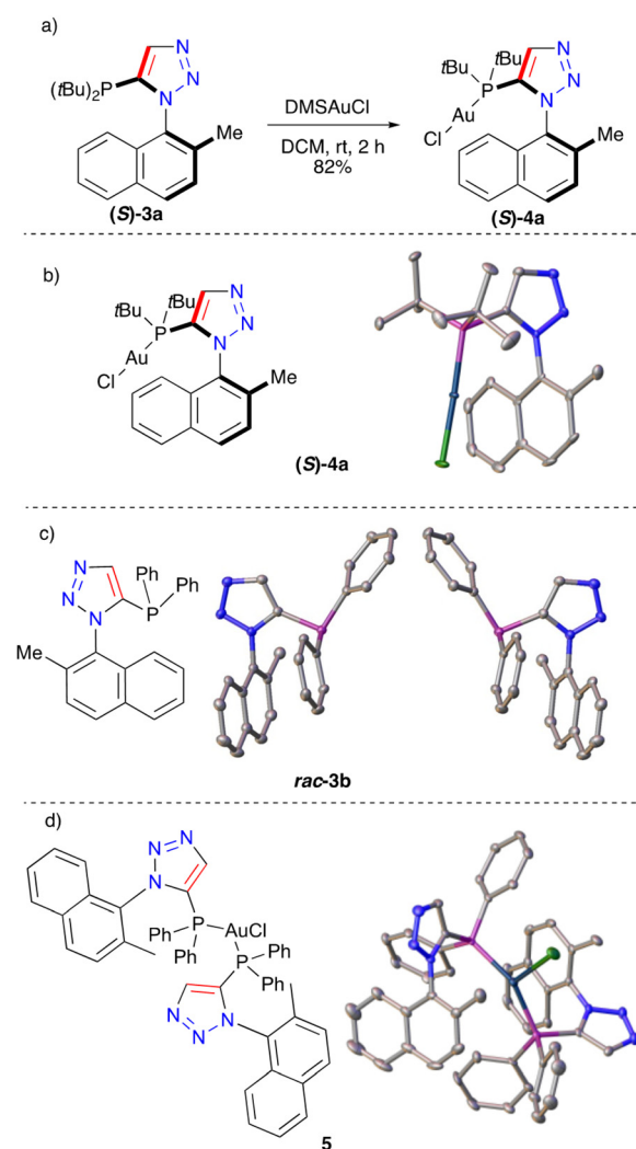
Fig. 3 (a) Synthesis of a single enantiomer gold(i) chloride complex (b) single-crystal X-ray diffraction structure of (S)\text{-4a} . Ellipsoids are drawn at the 50% probability level. A molecule of DCM has been omitted for clarity. Hydrogen atoms omitted for clarity. (c) Molecules from the crystal structure of rac-3b with ellipsoids drawn at the 50% probability level. Symmetry codes used to generate the equivalent atoms: (i) x, y, z . (ii) 1 - x, 1 - y, 1 - z . Hydrogen atoms omitted for clarity. (d) Single-crystal X-ray diffraction structure of homo-chiral complex 5 . Ellipsoids are drawn at the 50% probability level. A molecule of DCM has been omitted for clarity. Hydrogen atoms have been omitted for clarity.
