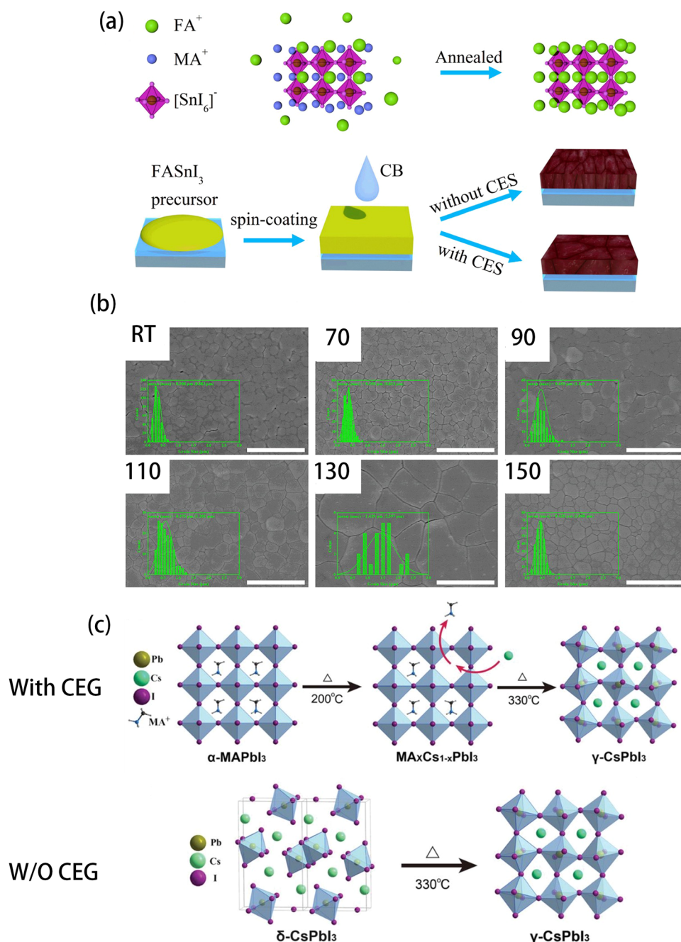
Fig. 9 (a) Schematic diagram of the cation exchange strategy (CES) method. (b) Top-view SEM images of FAcAc-RT, FAcAc-70 °C, FAcAc-90 °C, FAcAc-110 °C, FAcAc-130 °C, and FAcAc-150 °C perovskite films. The scale bar is 2 μm. Reproduced from ref. 108 with permission from American Chemical Society, copyright 2021. (c) Illustration of the CsPbI3 crystal formation using the cation exchange growth (CEG) method and control method. Reproduced from ref. 112 with permission from Wiley-VCH, copyright 2019.
