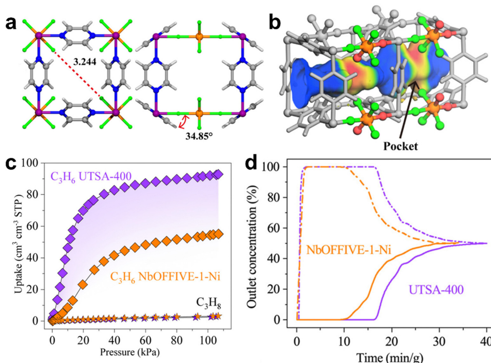
Fig. 14 (a) Crystal structure of UTSA-400. (b) Connolly surface of UTSA-400 mapped with electrostatic potential with a probe of 1.2 Å. (c) Single-component adsorption isotherms of C 3 H 6 and C 3 H 8 for UTSA-400 and NbOFFIVE-1-Ni at 298 K. (d) Breakthrough curves for NbOFFIVE-1-Ni and UTSA-400 for an equimolar binary mixture of C 3 H 6 (solid line)/C 3 H 8 (dashed line) at 298 K and 1 bar. Reprinted with permission from ref. 151. Copyright 2023 American Chemical Society.
