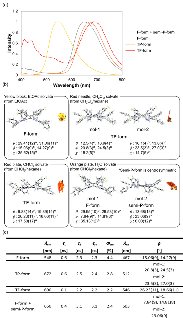
Fig. 4 (a) Emission spectra of each conformation of 1c in the solid state. (b) ORTEP drawings of 1c [F-form in EtOAc solvate (recrystallised from EtOAc), TP-form in \text{CH}_2\text{Cl}_2 solvate (recrystallised from \text{CH}_2\text{Cl}_2/\text{hexane} ), TF-form in \text{CHCl}_3 solvate (recrystallised from \text{CHCl}_3/\text{hexane} ), and those in which the F- and semi-P-forms exist as two crystallographically independent molecules in \text{H}_2\text{O} solvate (recrystallised from \text{CHCl}_3/\text{hexane} )]. Each of them was classified by the difference in dihedral angle \theta , \phi , and \chi for which emission spectra were measured. The solvent molecules are omitted for clarity. (c) Luminescence properties and dihedral angle \phi of each conformation of 1c were recorded in the solid state. All crystals were excited at 380 nm. Emission lifetimes were detected at the longer emission maximum. \lambda_{\text{ex}} is the value of the peak in the excitation spectra of 1c .
