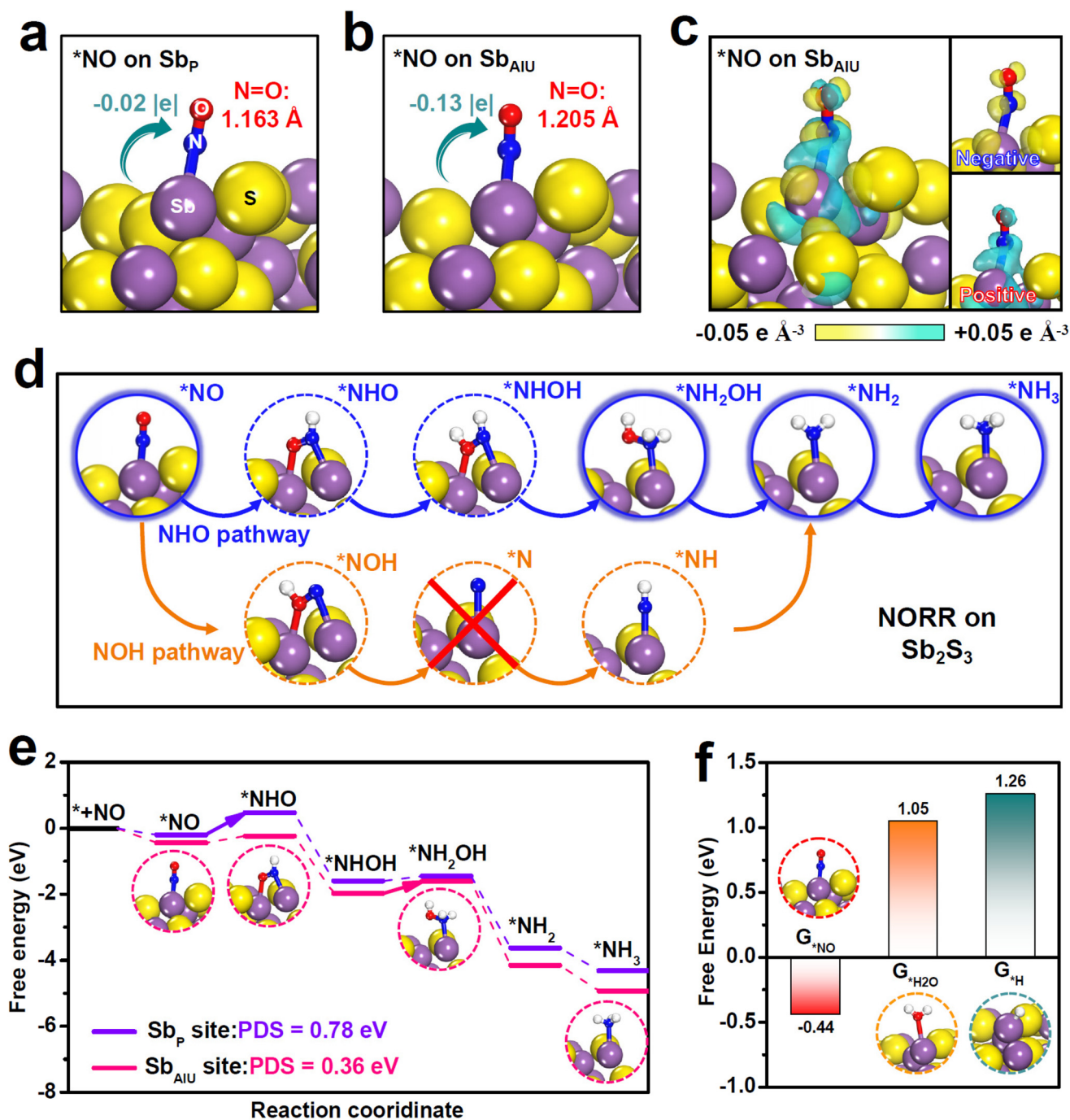
Fig. 3 (a and b) Atomic structures of absorbed NO on (a) the Sb_P site and (b) the Sb_{AIU} site of Sb_2S_3 . (c) Charge density difference of NO on the Sb_{AIU} site (yellow: accumulation; cyan: depletion). (d) Schematic of two NORR pathways (NHO and NOH) on Sb_2S_3 . (e) Free energy profiles of the NORR process (NHO pathway) on Sb_P and Sb_{AIU} . (f) Binding free energies of *H_2O , *H and *NO on Sb_{AIU} .
