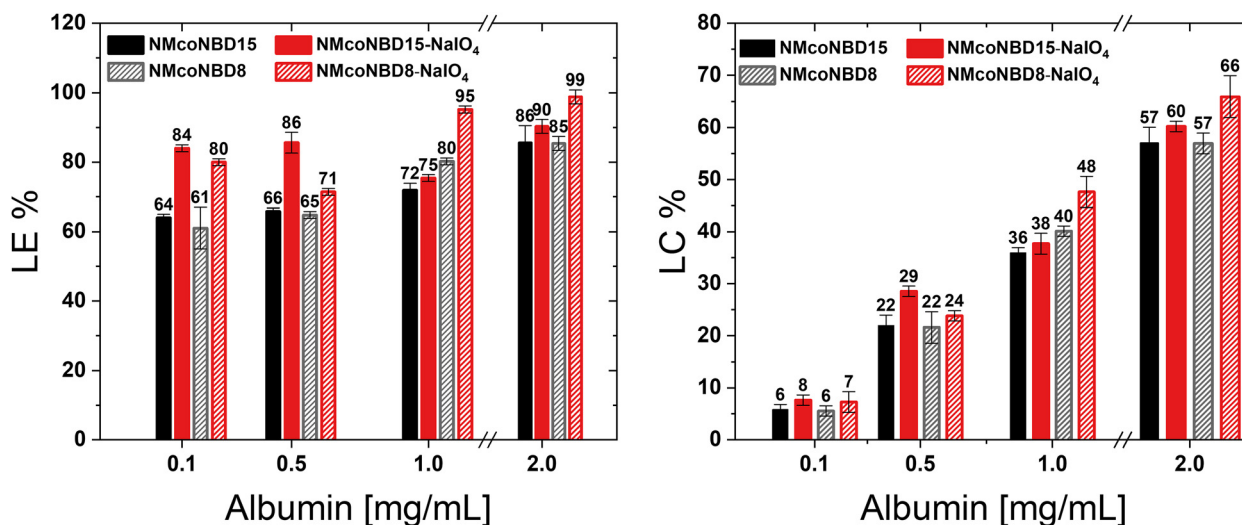
Fig. 3 Loading efficiency (LE%) and Loading capacity (LC%) of BSA-FITC into pristine p-NIPAm-co-NIPAm-BIS-DAT NGs (black/grey) and NGs modified with periodate (red).
