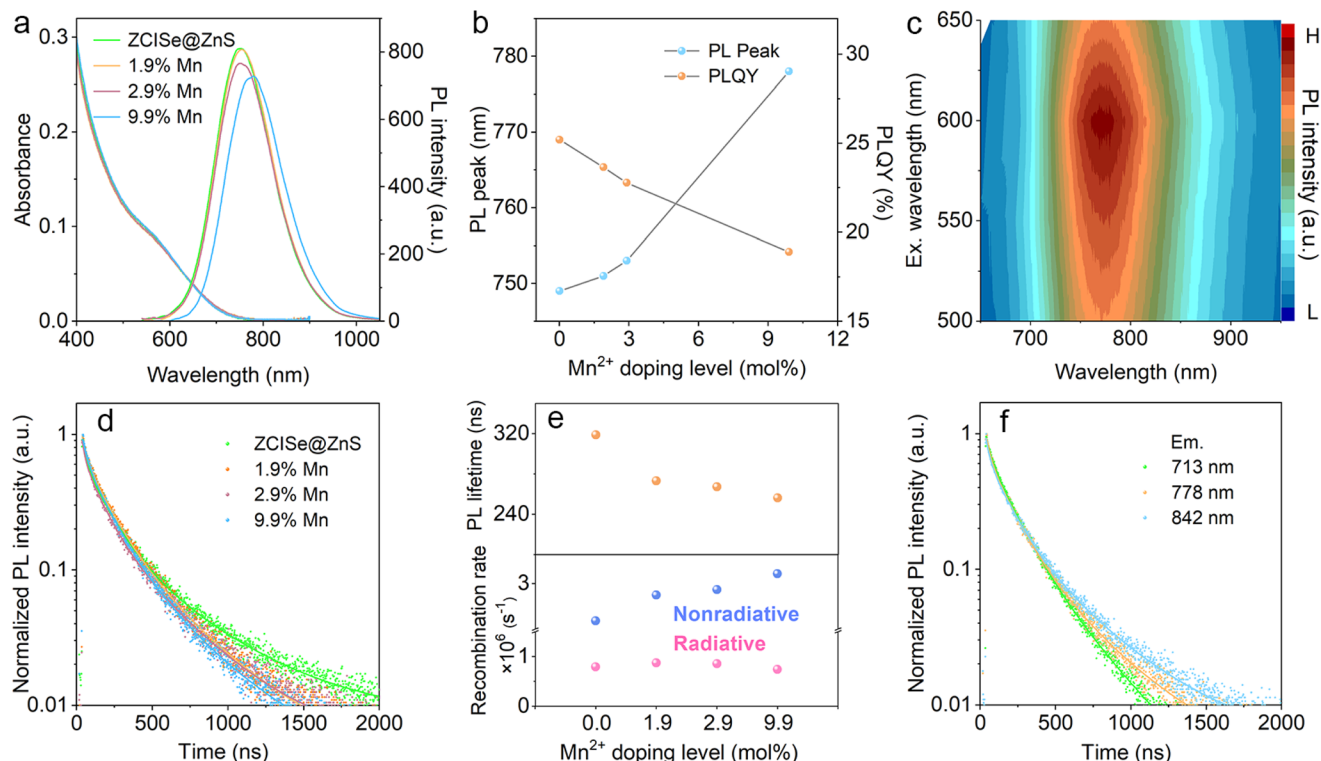
Fig. 1 (a) PL and absorption spectra of ZCISe@ZnS:Mn QDs with different Mn 2+ doping levels, (b) the evolution of the PL peak and PLQY of the QDs against the Mn 2+ doping level, (c) PL spectra recorded by excitation at different wavelengths for ZCISe@ZnS:Mn QDs with a Mn 2+ doping level of 9.9%, (d) time-resolved PL decay curves of ZCISe@ZnS:Mn QDs with different Mn 2+ doping levels, (e) the average lifetime and non-radiative/radiative recombination rates as a function of the Mn 2+ doping level, and (f) time-resolved PL decay curves of ZCISe@ZnS:Mn QDs with a Mn 2+ doping level of 9.9% at different emission wavelengths.
