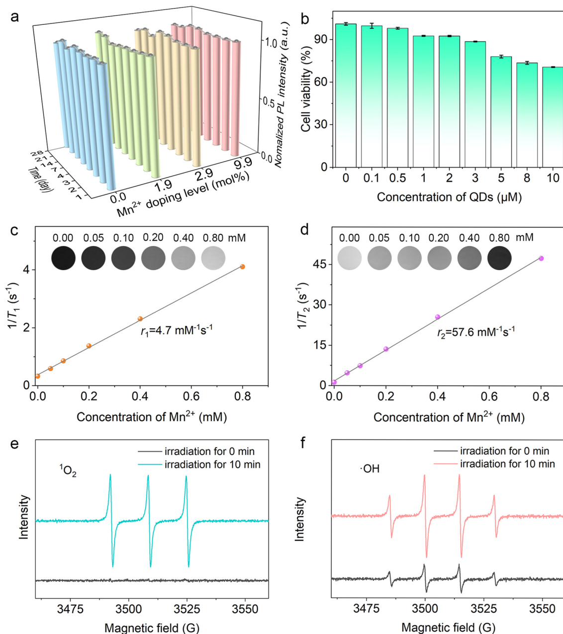
Fig. 3 (a) Temporal evolutions of PL intensity of ZnCdSe@ZnS:Mn QDs with different Mn 2+ doping levels, (b) cell viability of MCF-7 cells recorded after being treated with ZnCdSe@ZnS:Mn (doping level of 9.9%) QDs, the longitudinal relaxation rate (c) and transverse relaxation rate (d) against the concentration of Mn 2+ in doped QDs with the MR contrast images of aqueous solutions containing QDs (doping level of 9.9%) shown in the insets, and EPR spectra of ZnCdSe@ZnS:Mn (doping level of 9.9%) QDs for detecting 1 O 2 (e) and ·OH (f) with or without light irradiation (638 nm, 0.72 W cm -2 ).
