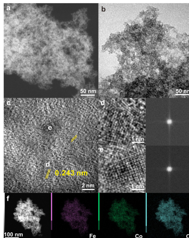
Fig. 2 TEM characterization of high-crystalline FeCo hydroxides. (a) STEM image, (b) TEM image, (c–e) HR-TEM images, and (f) EDX elemental mapping images.
