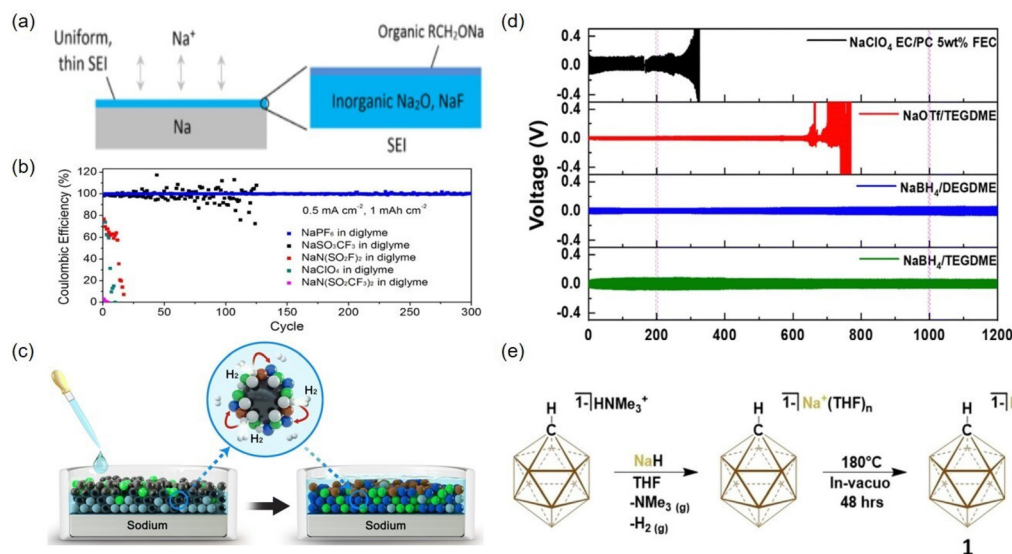
Fig. 6 (a) The schematic diagram of the SEI layer formed on the Na metal surface using \text{NaPF}_6 in the electrolyte. (b) The CE comparison of SMBs with various electrolyte salts in diglyme. 60 (c) The proposed formation mechanism of SEI layer on Na anode in \text{NaBH}_4 /diglyme electrolyte. (d) The cycle performance of Na||Na symmetric cells in the electrolytes of (black) \text{NaClO}_4 EC/PC + 5 wt% FEC, (red) \text{NaOTf}/\text{TEGDME} , (blue) \text{NaBH}_4/\text{diglyme} , and (green) \text{NaBH}_4/\text{TEGDME} . 108 (e) Convenient preparation process of \text{Na1} by the deprotonation of [\text{HNMe}_3]^+[\text{HCB}_{11}\text{H}_{11}]^- with \text{NaH} . 109 (Reprinted with permission from ref. 60, 108 and 109. Copyright 2015 American Chemical Society, Copyright 2022 Royal Society of Chemistry and Copyright 2022 Wiley-VCH GmbH).
