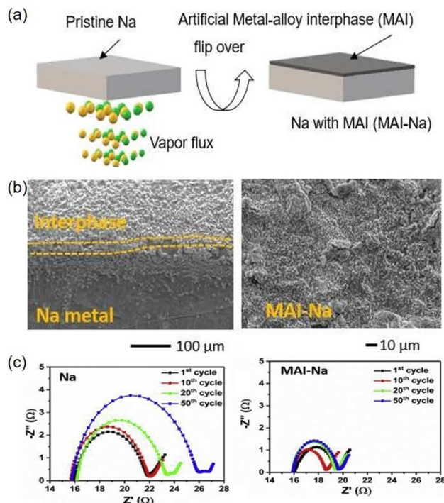
Fig. 11 (a) Graphical representation of the formation process of the artificial MAI on the Na metal interface. (b) Cross-sectional view of bare Na and MAI-Na interface. (c) The EIS of Na//Na cells without and with MAI after different stripping/plating cycles. 153 (Reprinted with permission from ref. 153. Copyright 2020 Elsevier B.V.).
