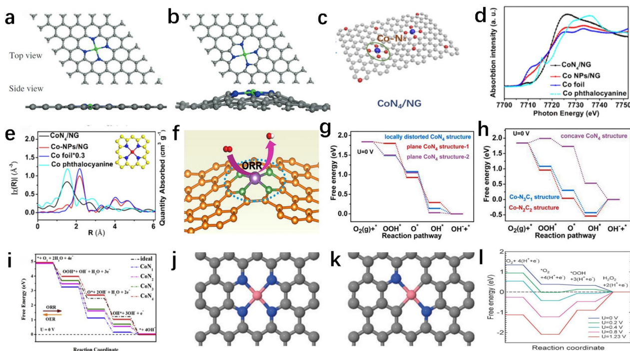
Fig. 10 (a and b) Top and side views of the optimized structures of CoN 4 -G(A) and CoN 4 -G(B). Reproduced with permission ref. 141. Copyright 2020, Wiley-VCH. (c-e) Schematic illustration, XANES Co K-edge spectra, and Fourier-transforms of Co K-edge spectra for CoN 4 /NG. Reproduced with permission ref. 142. Copyright 2018, Elsevier. (f) Distorted Co-N 4 structure. (g) Free energy diagram for the ORR on CoN 2 C 2 and CoN 3 C 1 . Reproduced with permission ref. 143. Copyright 2022, Elsevier. (h) Free energy diagrams for the ORR and OER pathways on CoN x (x = 1–4). Reproduced with permission ref. 144. Copyright 2019, Elsevier. (i) Schematic illustration of CoN 4 and CoN 2 . (j) Free energy diagram for the reduction of O 2 to H 2 O 2 on the CoN 4 defect. Reproduced with permission ref. 145. Copyright 2019, Royal Soc Chemistry.
