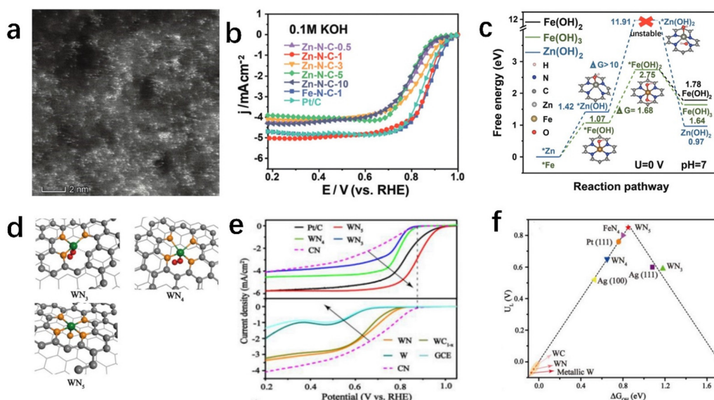
Fig. 16 (a and b) Aberration-corrected HAADF-STEM image and ORR polarization curve of the Zn-N-C-1. (c) Free-energy diagrams for \text{Zn(OH)}_2 , \text{Fe(OH)}_2 , and \text{Fe(OH)}_3 . Reproduced with permission ref. 183. Copyright 2019, Wiley-VCH. (d and e) Schematic models and comparison of the ORR performances of \text{WN}_3 , \text{WN}_4 , and \text{WN}_5 . (f) Illustration of the limiting potential ( U_L ) "volcano" as a function of the change in \Delta G_{\text{OH}} . Reproduced with permission ref. 184. Copyright 2019, Elsevier.
