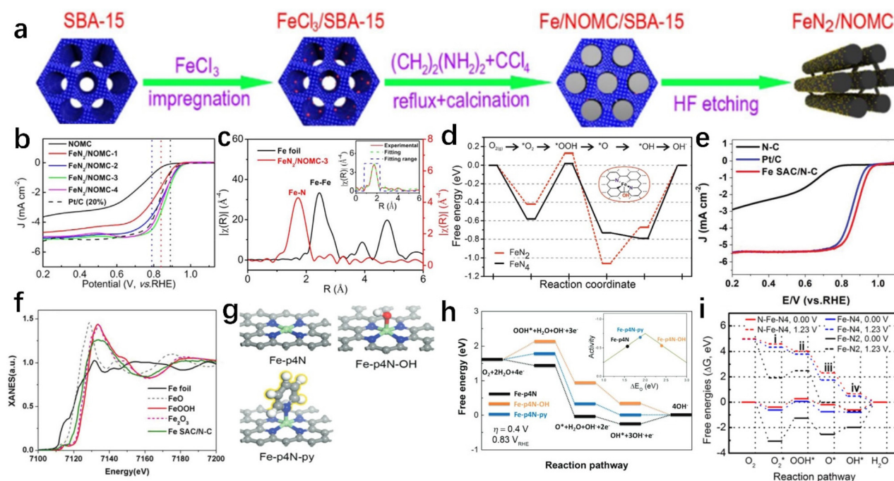
Fig. 7 (a–d) The synthetic procedure, ORR polarization, EXAFS spectra, and free energy diagram for \text{FeN}_2/\text{NOMC} . Reproduced with permission ref. 126. Copyright 2017, Elsevier. (e–h) LSV curves, XANES spectra, three models with various coordination environments, and free energy diagrams of Fe SAC/N-C. Reproduced with permission ref. 128. Copyright 2019, Wiley-VCH. (i) Free energy diagrams of the N-Fe-N 4 , Fe-N 4 , and Fe-N 2 in acid media. Reproduced with permission ref. 129. Copyright 2017, American Chemical Society.
