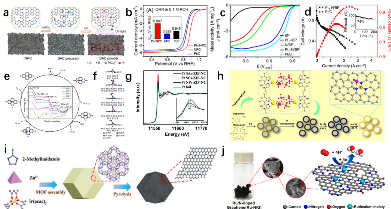
Fig. 5 (a and b) Schematic illustration, ORR polarization curves of Pt 1 /NPC. Reproduced with permission ref. 96. Copyright 2018, American Chemical Society. (c–f) RRDE polarization curves, the voltages and power densities of H 2 /O 2 fuel cells, the free energy diagram, side view, and bond lengths of Pt 1 -N/BP. Reproduced with permission ref. 97. Copyright 2017, Nature. (g) The XANES spectra of Pt SAs-ZIF-NC. Reproduced with permission ref. 98. Copyright 2020, Wiley-VCH. (h) The preparation of the PtNPNC. Reproduced with permission ref. 51. Copyright 2021, Wiley-VCH. (i) Schematic illustration of Ir/N-C. Reproduced with permission ref. 103. Copyright 2019, Wiley-VCH. (j) Illustration of Ru-N/G. Reproduced with permission ref. 105. Copyright 2017, American Chemical Society.
