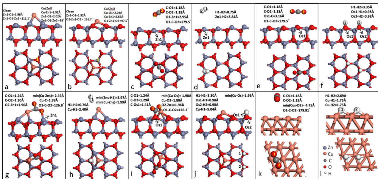
Fig. 2 The most stable geometry of Cu deposited at the fcc-site for (a) the clean ZnO(0001) and (b) ZnO(0001) surfaces. The most stable geometry of (c) CO 2 and (d) H 2 adsorbed on the clean surface of ZnO(0001); and the most stable geometry of (e) CO 2 and (f) H 2 adsorbed on the clean surface of ZnO(0001). The most stable geometry of (g) CO 2 and (h) H 2 adsorbed on Cu/ZnO(0001); the most stable geometry of (i) CO 2 and (j) H 2 adsorbed on the Cu/ZnO(0001) system; the most stable geometry of (k) CO 2 and (l) H 2 adsorbed on metallic Cu(111).
