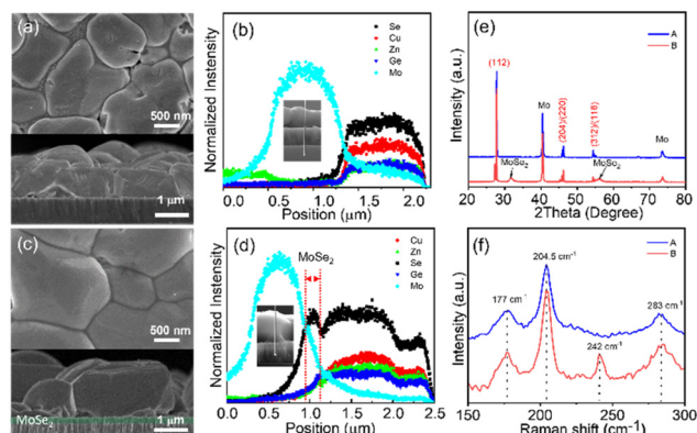
Fig. 3 (a–d) Surface and cross-sectional SEM images, and EDX line profiles of CZGSe absorbers (a and b: CZGSe-A; c and d: CZGSe-B). (e and f) XRD patterns and Raman spectra of CZGSe-A and CZGSe-B.
