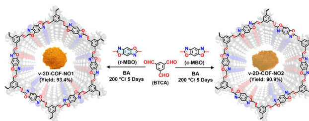
Fig. 5 Synthesis of isomeric v-2D-COF-NO1 and v-2D-COF-NO2 via the aldol-type polymerization between benzene-1,3,5-tricarbaldehyde (BTCA) and 2,6-dimethylbenzo[1,2- b :4,5- b' ]bisoxazole (t-MBO) or 2,6-dimethylbenzo[1,2- b :5,4- b' ]bisoxazole (c-MBO). Reproduced with permission from ref. 26. Copyright 2022, American Chemical Society.
