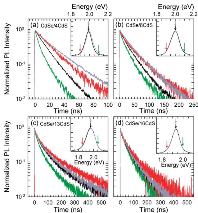
Fig. 5 PL decay curves of CdSe/CdS QD solution (gray lines) and film (red, black and green lines) with a (a) 4, (b) 8, (c) 13, and (d) 16 monolayer CdS shell. Inset: The PL spectrums of CdSe/CdS QD solution (solid black curves) and film (dashed gray curves). The PL decay curves are collected at the emission energies indicated by the arrows in the insets. Reproduced with permission. 62 Copyright 2012, American Chemical Society.
