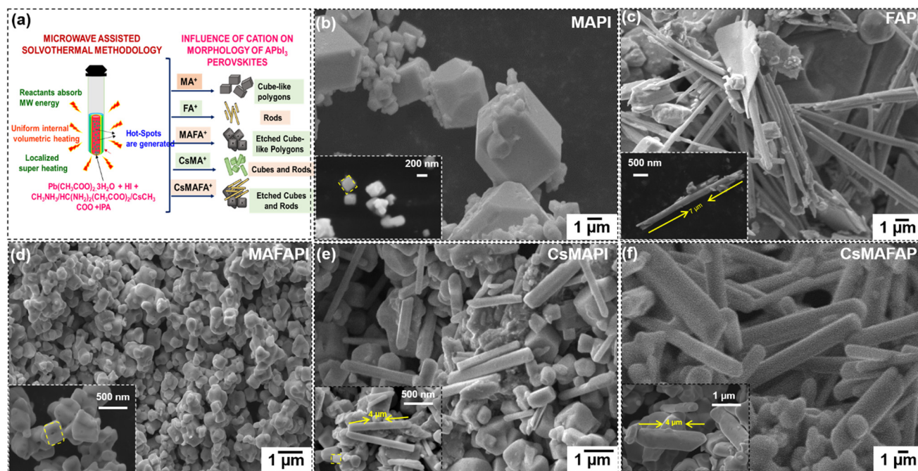
Fig. 10 (a) Schematic illustration of influence of cation-induced morphology change in \text{APbI}_3 ( \text{A} = \text{MA}^+ , \text{FA}^+ , \text{MAFA}^+ , \text{CsMA}^+ and \text{CsMAFA}^+ ) metal halide perovskites. (b–f) SEM images of various cations doped in the A-site of \text{APbI}_3 metal halide perovskites induced morphology changes (b) cube-like polyhedrons when \text{A} = \text{MA}^+ (c) rods observed with \text{A} = \text{FA}^+ , (d) truncated cube-like polyhedrons when \text{A} = \text{MAFA}^+ (e) mixed morphology of cubes with rods when \text{A} = \text{CsMA}^+ and (f) mixed morphology of rods and truncated cube-like polyhedrons when \text{A} = \text{CsMAFA}^+ in the A-site of \text{APbI}_3 metal halide perovskites.
