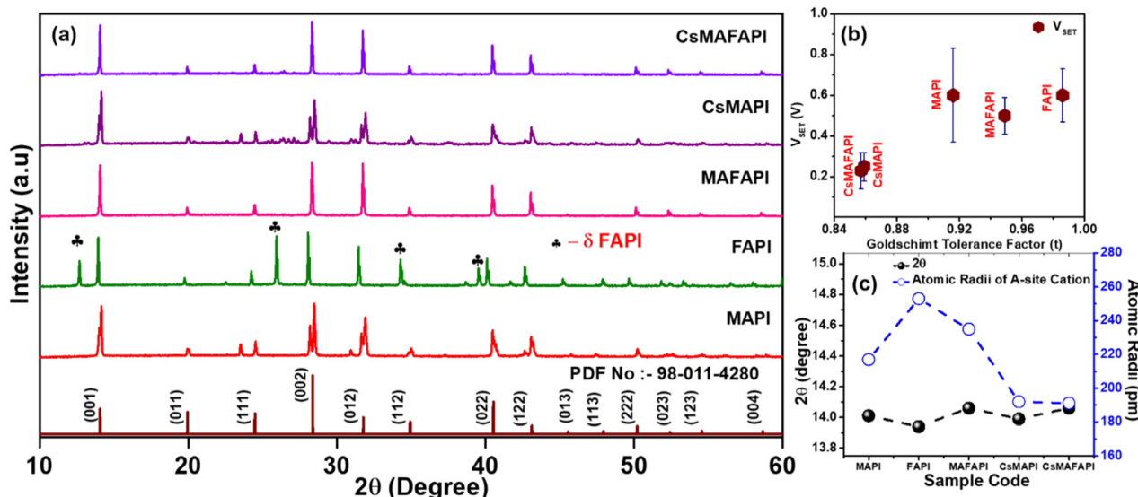
Fig. 1 (a) XRD pattern of the MW-ST synthesized APbI 3 ( A = \text{MA}^+ , \text{FA}^+ , \text{MAFA}^+ , \text{CsMA}^+ and \text{CsMAFA}^+ ) metal halide perovskite powders depicting the (b) variation of Goldschmidt tolerance factor with the operation V_{\text{SET}} voltage and (c) the shift of 2\theta = 14^\circ , with respect to the atomic radii of the substitutional cations.
