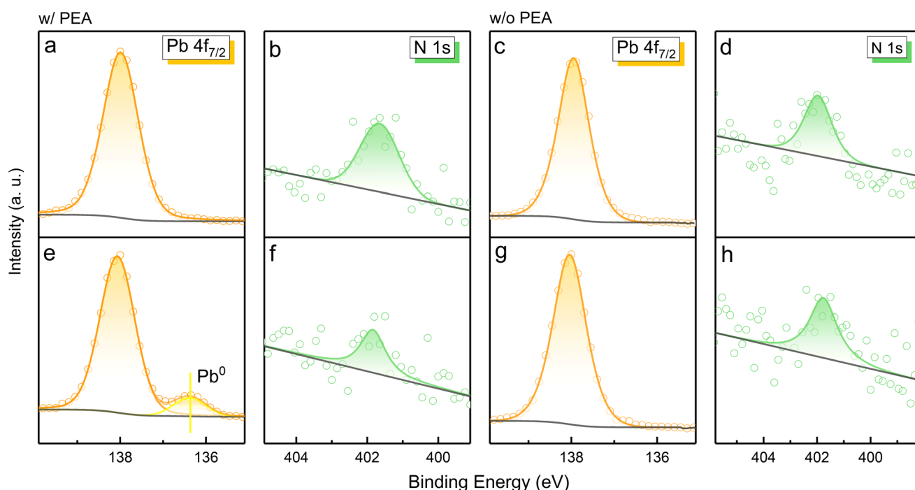
Fig. 2 Evolution of the chemical state and element content in 3D and reduced-dimensional \text{CsPbBr}_3 films. In situ XPS spectra from the orbitals of (a) \text{Pb } 4f_{7/2} and (b) \text{N } 1s in perovskite film w/PEA, and (c) \text{Pb } 4f_{7/2} and (d) \text{N } 1s in perovskite film w/o PEA before electron radiation; (e) \text{Pb } 4f_{7/2} and (f) \text{N } 1s in perovskite film w/PEA, and (g) \text{Pb } 4f_{7/2} and (h) \text{N } 1s in perovskite film w/o PEA after electron radiation for 3 h.
