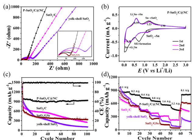
Fig. 3 Electrochemical performance of \text{P-SnO}_2/\text{C@NC} , \text{SnO}_2/\text{C} , yolk-shell \text{SnO}_2 and \text{SnO}_2/\text{GS} electrodes. (a) EIS spectra of \text{P-SnO}_2/\text{C@NC} , \text{SnO}_2/\text{C} , yolk-shell \text{SnO}_2 and \text{SnO}_2/\text{GS} electrodes. (b) CV curves of \text{P-SnO}_2/\text{C@NC} electrodes in the initial three cycles between 5 mV and 3.0 V at a scan rate of 0.1 \text{mV s}^{-1} . (c) Cycling performance and (d) rate capability of \text{P-SnO}_2/\text{C@NC} , \text{SnO}_2/\text{C} , yolk-shell \text{SnO}_2 and \text{SnO}_2/\text{GS} electrodes.
