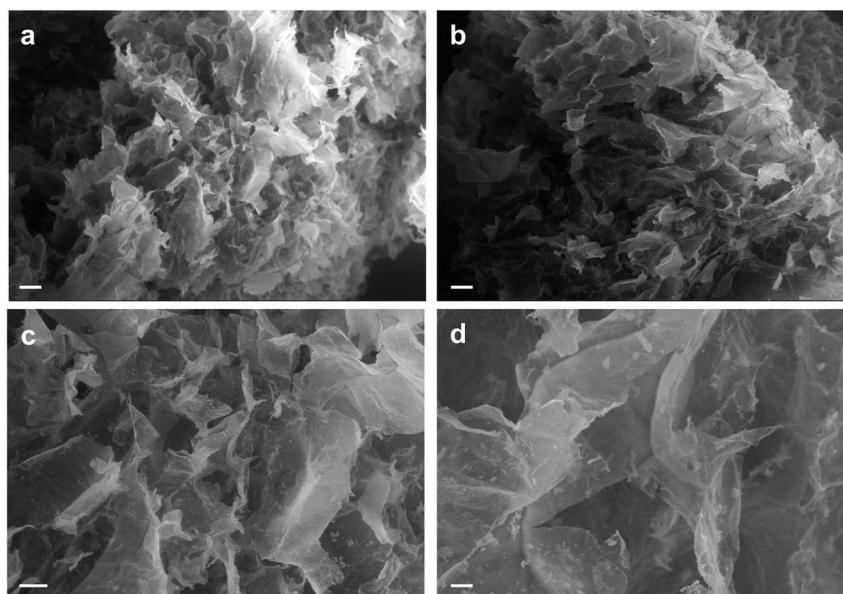
Fig. 4 SEM analysis of AC hydrogels loaded with Au NRs (a and c) and neat AC hydrogels (b and d). Scale bars: 200 \mu\text{m} (a and b); 100 \mu\text{m} (c and d).
