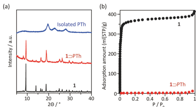
Fig. 3 (a) XRPD patterns of 1 , 1 \supset PTh, and PTh liberated from 1 . (b) \text{N}_2 adsorption isotherms of 1 and 1 \supset PTh at 77 K ( 1 ; S_{\text{BET}} = 1447 \text{ m}^2 \text{ g}^{-1} , 1 \supset PTh; S_{\text{BET}} = 4 \text{ m}^2 \text{ g}^{-1} ).
