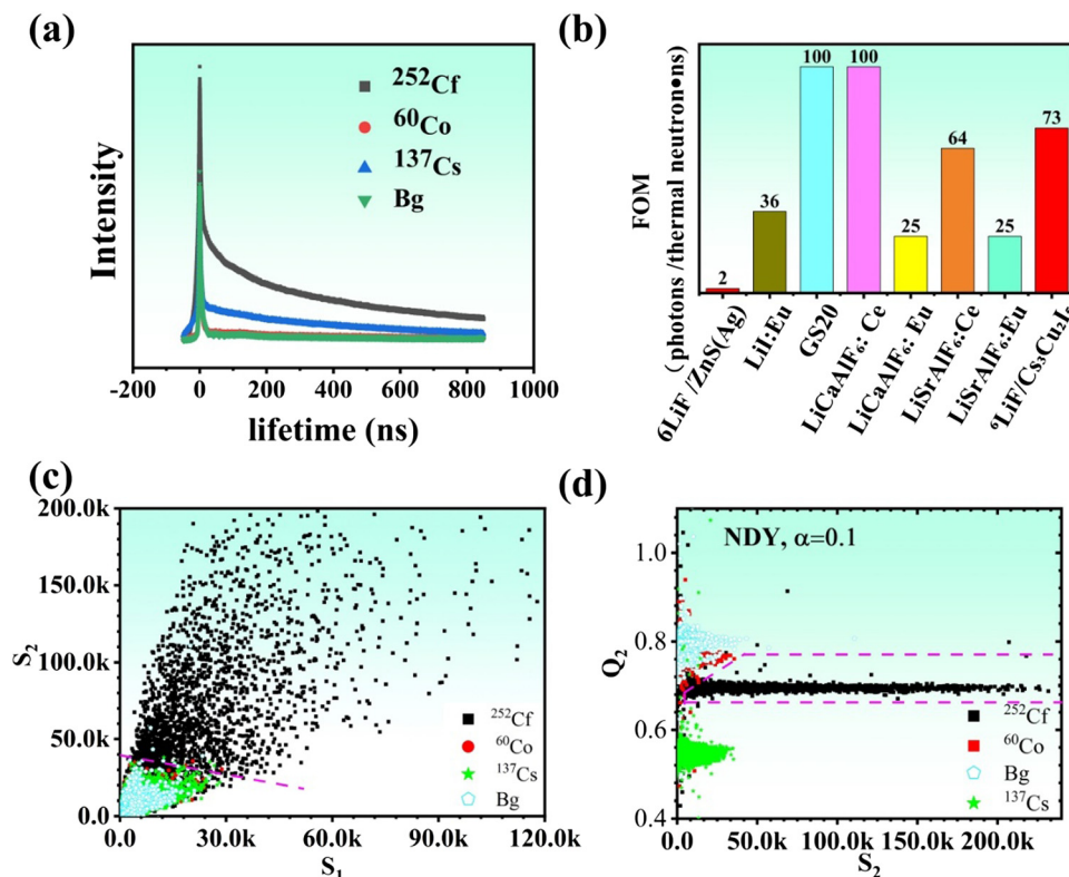
Fig. 4 RL properties of the composite ( \text{Cs}_3\text{Cu}_2\text{I}_5 ) _6 LiF/PMMA = 1 : 1 : 2): (a) decay curves under the irradiation of ^{60}\text{Co} , ^{252}\text{Cf} and ^{137}\text{Cs} and backgrounds, (b) the FoM in comparison with several well-known neutron scintillators. Neutron-gamma discrimination (NGD) films calculated by two methods, (c) conventional two-feature S_1 - S_2 plot and (d) gamma-embedded non-negative matrix factorization (GNMF) method. In (d) Q_2 is the second vector of projected matrix Q_2 = H(L)V , H = 1/(1 + \alpha L) is the network dynamics filter, L is the Laplacian operator of the event graph, \alpha is a hyperparameter, and V is the signal matrix. 44
