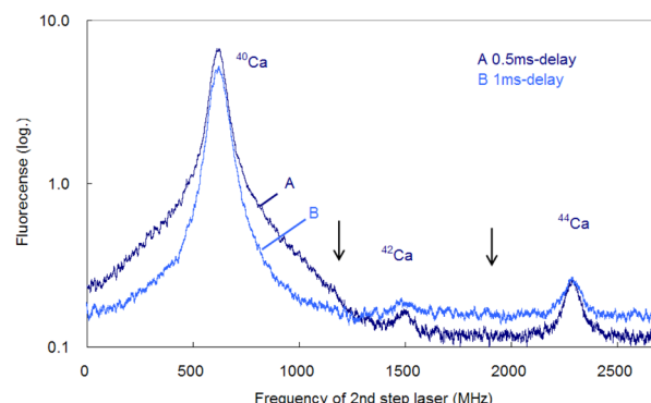
Fig. 11 Comparison of the isotope-selective fluorescence spectra measured at (a) 0.5 ms delay and (b) 1 ms delay. The second-step laser frequency was scanned from about -600 MHz of the resonance of ^{40}\text{Ca} to a high frequency, and the first-step laser frequency was rapidly switched from the resonance of ^{40}\text{Ca} to those of ^{42}\text{Ca} and ^{44}\text{Ca} at about 1.2 GHz and 2.0 GHz (marked with arrows), respectively.
