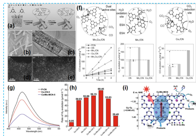
Fig. 27 (a) Synthesis of the Mn 1 Co 1 /CN catalyst. (b) SEM and (c) TEM images of Mn 1 Co 1 /CN. (d) AC HAADF-STEM image of (d) Mn 1 /CN and (e) Mn 1 Co 1 /CN. (f) Photocatalytic activities of samples with double single-atom active sites for CO 2 reduction. 110 (g) Photoluminescence spectra of P-CN, Co-CN-5, and Co/Mo-MCN-5. (h) Photocatalytic H 2 evolution rate of the as-prepared materials. (i) Photocatalytic mechanism scheme of Co/Mo-MCN under visible light irradiation. 111
