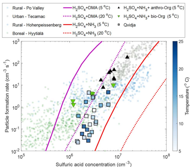
Fig. 3 Particle formation rate ( J_{1.5} ) as a function of \text{H}_2\text{SO}_4 concentration, daily averages (12:00–16:00 LT) – squares, colored with ambient temperature (average temperature is 13 °C). Parametrization based on chamber measurements of \text{H}_2\text{SO}_4 + \text{NH}_3 (2 ppbv) ammonia at 5 °C (solid red line) and 20 °C (dotted red line) is shown. 70 Similarly, parametrization based on chamber measurements of \text{H}_2\text{SO}_4 + dimethylamine (DMA – 4 pptv) at 5 °C (solid magenta line) and 20 °C (dotted magenta line) is shown. 70 Green triangles are \text{H}_2\text{SO}_4 + \text{NH}_3 (0.1–1 ppbv) at 5 °C in the presence of constant monoterpenes ( \alpha -pinene and \Delta -3-carene) and \text{NO}_x from Lehtipalo et al. 67 Black triangles are \text{H}_2\text{SO}_4 + \text{NH}_3 (1–2 ppbv) in the presence of anthropogenic organics. 70 Filled translucent points in the background are atmospheric measurements from the boreal forest (green), rural locations 90,91 (pink) and polluted environments (gray). 92 The measured particle formation rates from Qvidja are at 1.5 nm, while those from chamber measurements are measured at 1.7 nm 51 and extrapolated to 1.5 nm using the Kerminen and Kulmala equation. 93 The particle formation rates from atmospheric observations are also reported at 1.5 nm.
