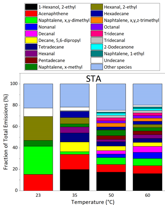
Fig. 6 Evolution of VOC emission composition in % for the species accounting for more than 75% of VOC emissions ( \text{EF} > 3.49 \mu\text{g m}^{-2} \text{ h}^{-1} for STA asphalt mixtures) as a function of temperature, as measured by GC-MS/FID under dry (RH = 0.1%) and dark conditions, for the STA3 fresh asphalt sample.
