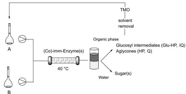
Scheme 2 Flow bioprocessing of HES and RT. Solution A: 10 g\ L^{-1} HES or RT in TMO. Solution B: HEPES buffer, 0.05 M, pH 7.5. Co-imm-enzyme(s): imm-RN (5 mg g_{\text{resin}}^{-1} ) or HOR (1 mg g_{\text{resin}}^{-1} ) or imm-RN-HOR (5 mg RN g_{\text{resin}}^{-1} , 1 mg HOR g_{\text{resin}}^{-1} ). T = 40\ ^\circ\text{C} .
