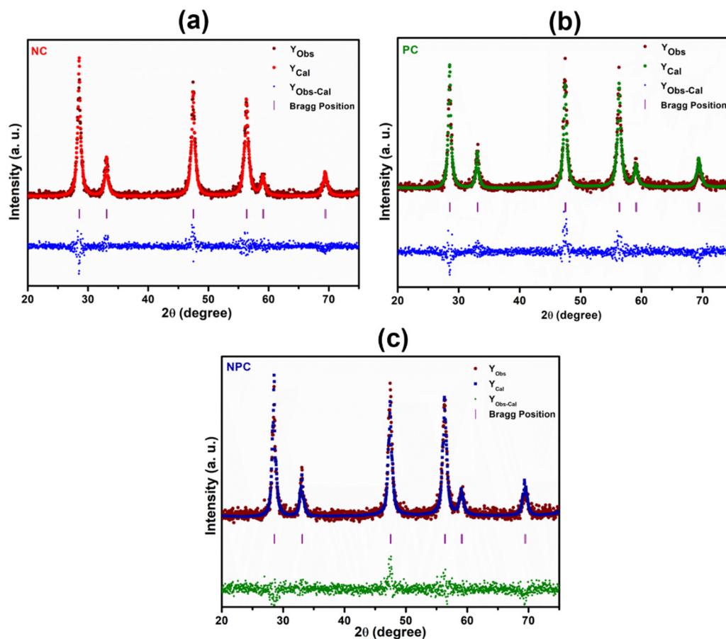
Fig. 2 Rietveld refinement XRD patterns of NC (a), PC (b), and NPC (c) catalysts. Difference between observed and calculated intensities ( Y_{obs-cal} ), calculated intensity ( Y_{cal} ) and observed intensity ( Y_{obs} ). Vertical lines indicate peak positions and differences.
