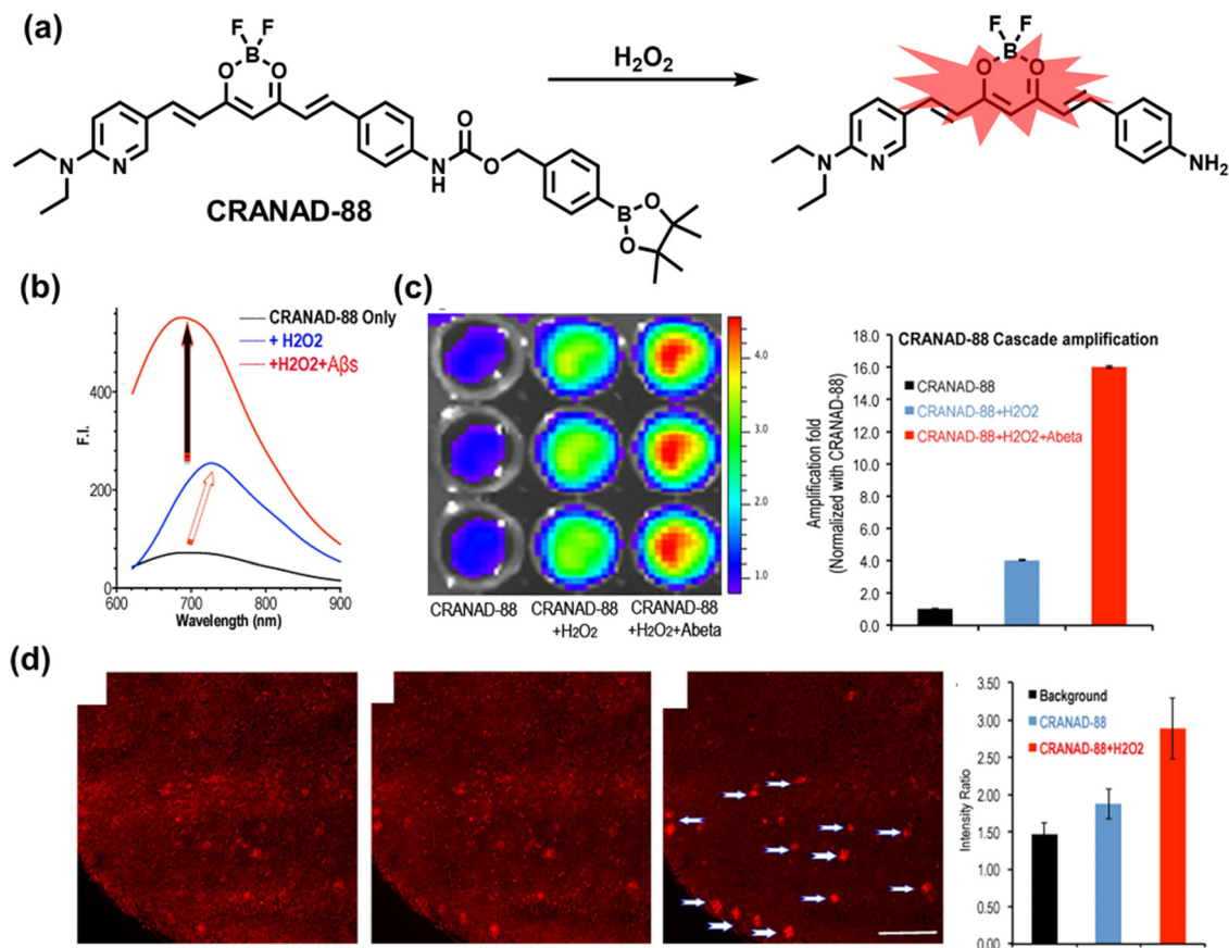
Fig. 22 (a) Structures of CRANAD-88 and reaction with \text{H}_2\text{O}_2 . (b) Fluorescence intensity changes of CRANAD-88 with \text{H}_2\text{O}_2 and with \text{H}_2\text{O}_2 + A \beta aggregates. (c) Cascade signal amplification validation of CRANAD-88 on a plate and quantitative analysis of the image. (d) \text{H}_2\text{O}_2 -treated/untreated brain sections were evaluated for staining using CRANAD-88 and quantification histograms. Reproduced with permission from ref. 207. Copyright (2016) Springer Nature.
