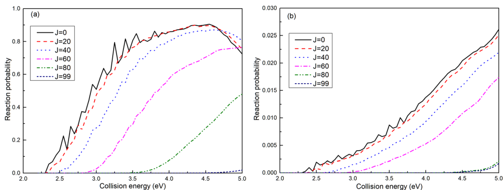
Fig. 4 Reaction probabilities of the \text{Ca}^+(4s^2S) + \text{H}_2(\text{X}^1\Sigma_g^+) \rightarrow \text{H}(\text{H}^2S) + \text{CaH}^+(\text{X}^1\Sigma^+) reaction calculated from adiabatic PES (a) and non-adiabatic PES (b).
