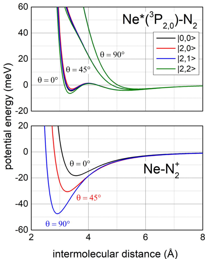
Fig. 13 Upper panel: The real part V_r of the optical potential with its dependence on the intermolecular distance, on the orientation angle \theta of \text{N}_2 and on the |\text{J}, \Omega\rangle quantum state of \text{Ne}^*(^3P_j) reagent. Intermediate panel: The anisotropic interaction potential in the exit channels. Lower panel: A basic configuration of the precursor state of \text{Ne}^*(^3P_j) + \text{N}_2 CHEMI in the collinear configuration of reagents (for more details see ref. 119).
